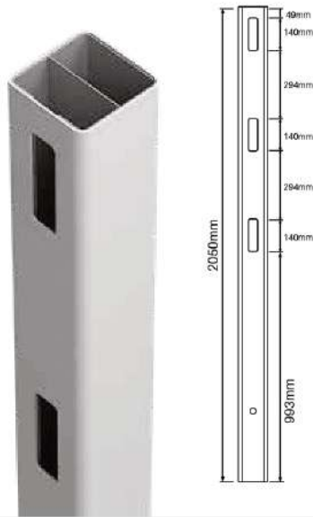
127MM X 127MM 1 way gate post – 3 Rail 2050MM LONG Order Code: HF-3RAIL-2050-1WGP
