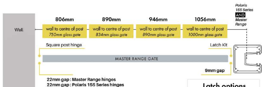
Master range square post hinge set Set of 2 MR-SPH-P/S/B
